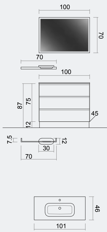
Encimera TIFF válvula Tiff con logo. / TIFF countertop TIFF valve with logo. / Plan TIFF Soupape TIFF avec logo.
