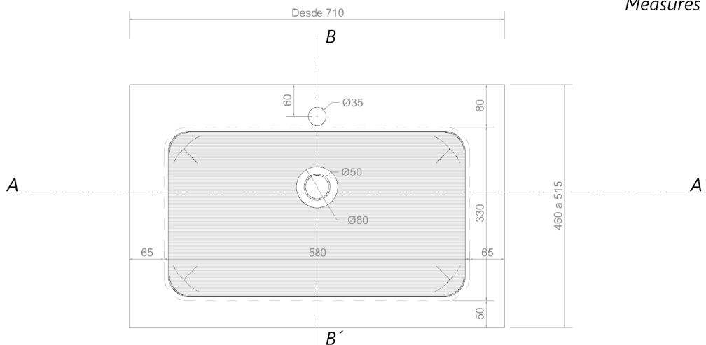
PLANTA PLANT
