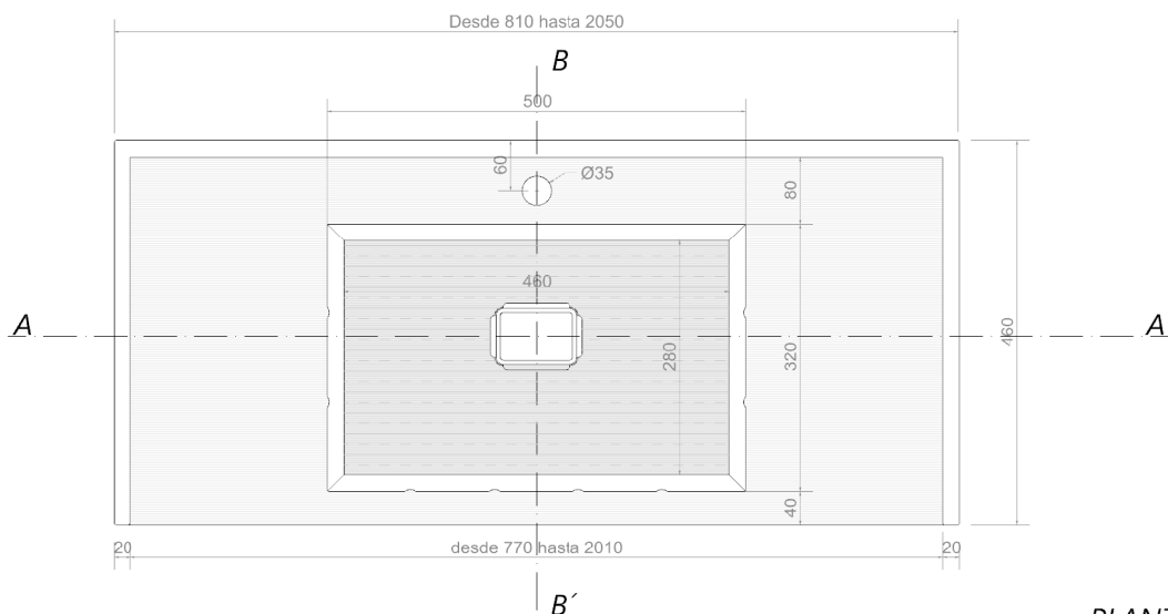
PLANTA PLANT
