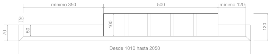
ALZADO FRONTAL FRONT SIDE
