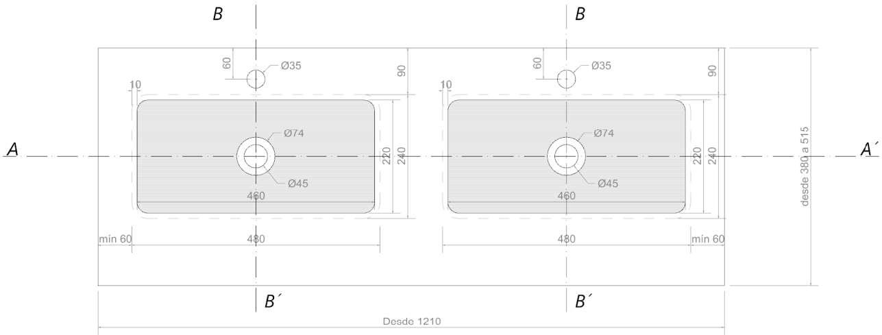
PLANTA PLANT
